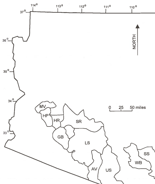
Figure 1. Regions of Arizona known to have undergone pumping subsidence. The regions shown are ground-water areas. Only a portion of each area has subsided. In McMullen Valley, subsidence has not been measured but has probably occurred. AV = Aora Valley; GB = Gila Bend Basin; HP = Harquahala Plain; HR = lower Hassayampa River valley; LS = lower Santa Cruz River basin; MV = McMullen Valley; SR = Salt River Valley; SS = San Simon Basin; US = upper Santa Cruz River basin; WB = Willcox Basin. Modified from Schumann and others (1986).
