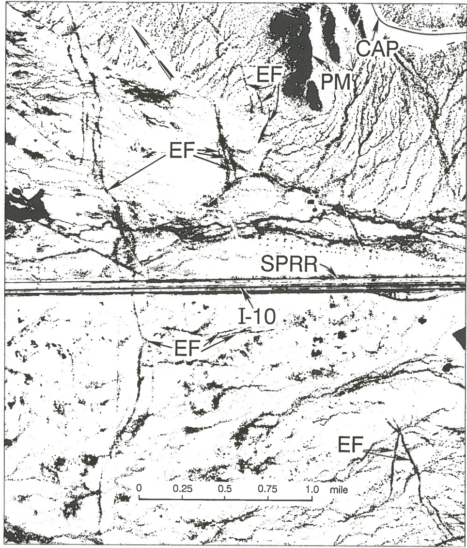
Figure 12. Aerial photograph taken in August 1987 of area southeast of Picacho in Pinal County. Dense vegetation growing along earth fissures makes them appear as dark lines. EF = earth fissure; PM = southern end of Picacho Mountains; CAP = Central Arizona Project aqueduct; SPRR = Southern Pacific Railroad; I-10 = Interstate Highway 10. Photo by Arizona Department of Transportation.
